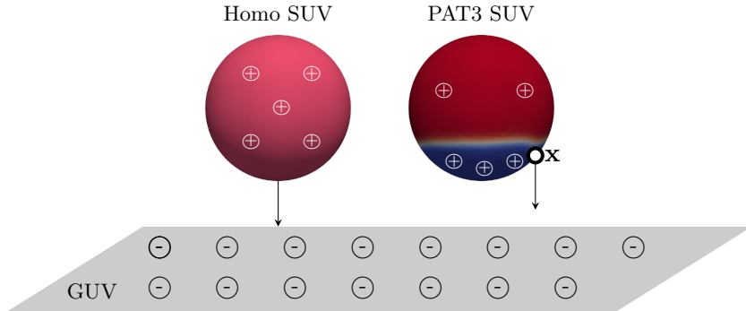
Figure 25: Relative positions of GUV, represented as a plane, and a positively charged SUV, homogeneous (sphere on the left) or phase-separated PAT3 SUV (sphere on the right), in a simulation. The L_o phase in the phase-separated SUV is colored in red, while the L_d phase is blue.
