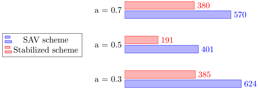
Figure 10: Phase separation on the sphere: computational time (in s) needed by the stabilized method in [115] and the SAV method with no time step adaptivity to complete the first 100 time steps of the simulations in Fig. 4 ( a = 0.5 ), 5 ( a = 0.3 ), and 6 ( a = 0.7 )
