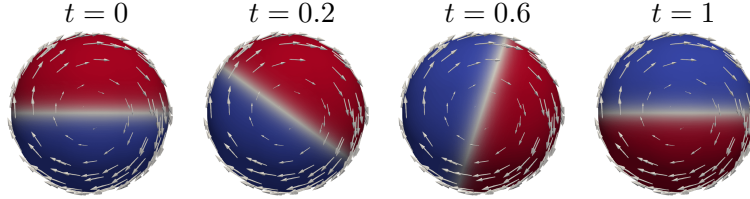
Figure 13: Evolution of the surface fraction c over time computed with mesh \ell = 5 .
